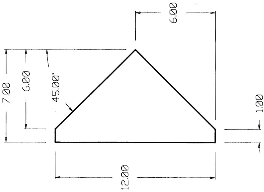
45° Fixture
