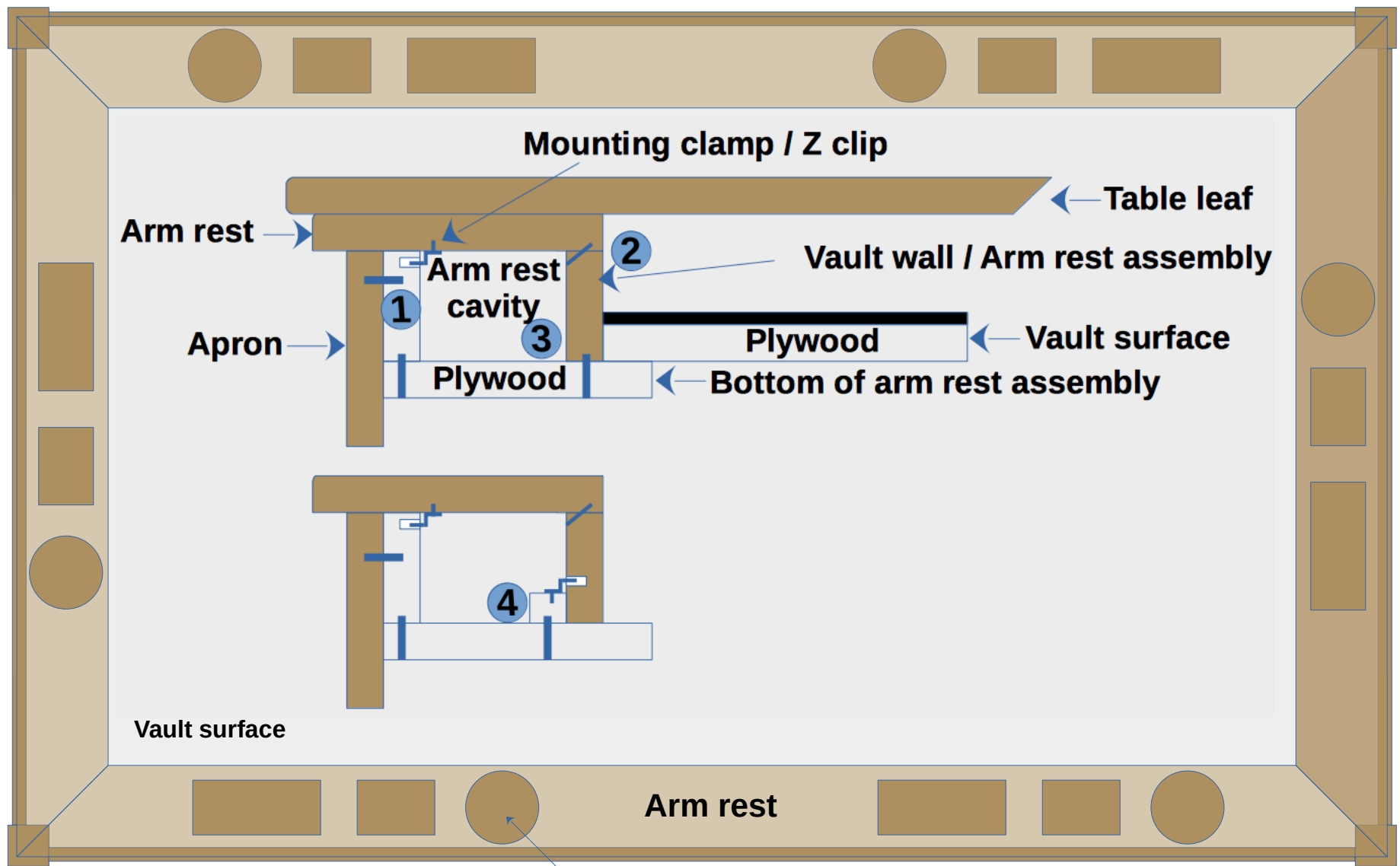
Arm rest cavities accessible from above through these holes
